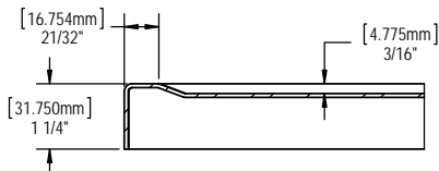
SECTION A-A SCALE 1 : 2 MARINE EDGE DETAIL
