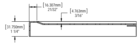
SECTION A-A SCALE 1:2 MARINE EDGE DETAIL
