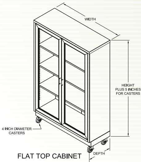
FLAT TOP CABINET
