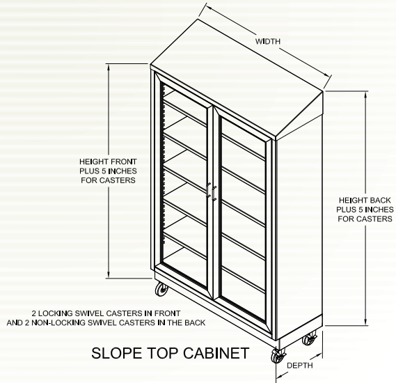
SLOPE TOP CABINET
